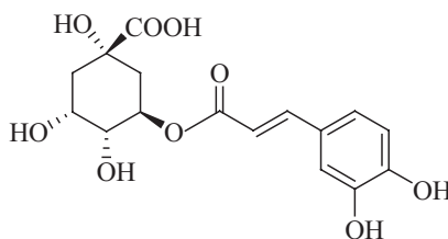
15. Chlorogenic acid
