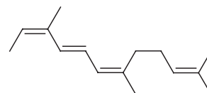
3. Farnesene
