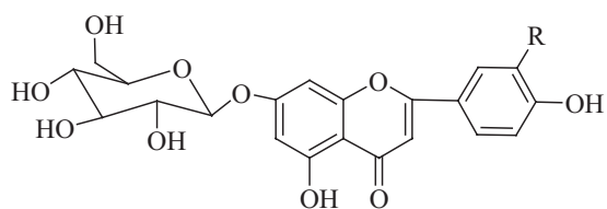
18. Apigenin-7-O-glucoside (R=H)
