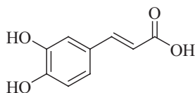
14. Caffeic acid
