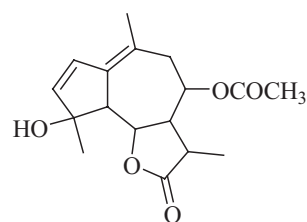
9. Matricin
