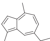
10. Chamazulene
