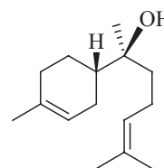
6. (-)- \alpha -bisabolol
